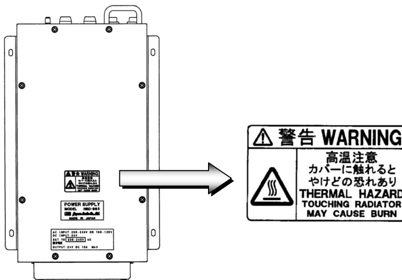
NBD-865 Power supply (Upper view)
