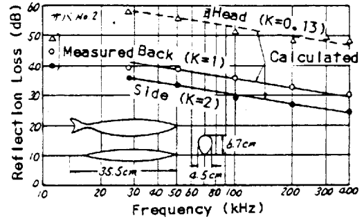
Reflection Loss (Mackerel No.2)
