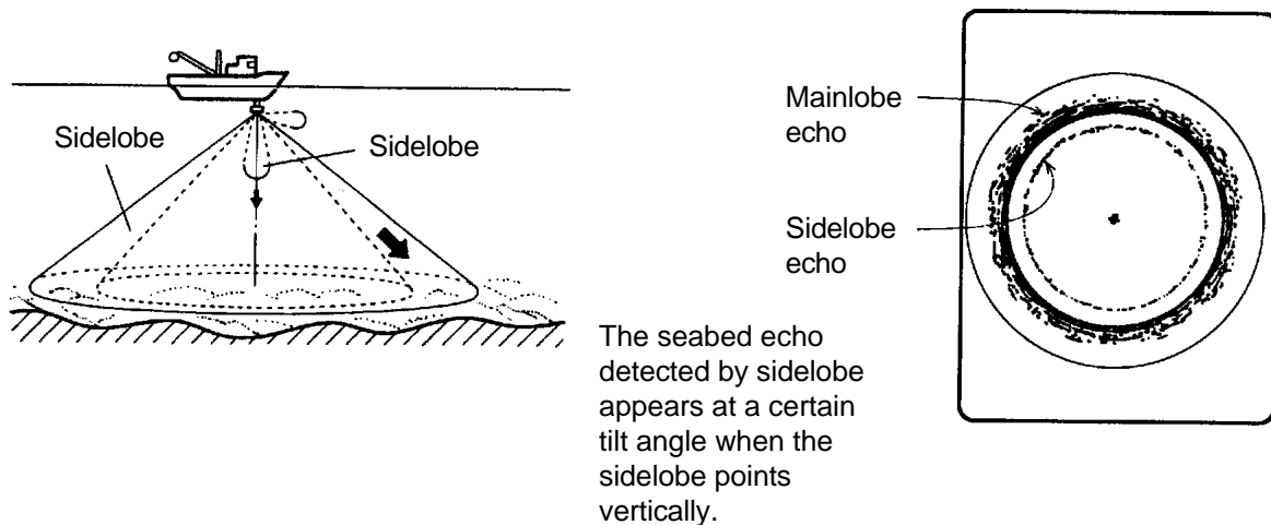
Figure 6-5 Sidelobe echoes
