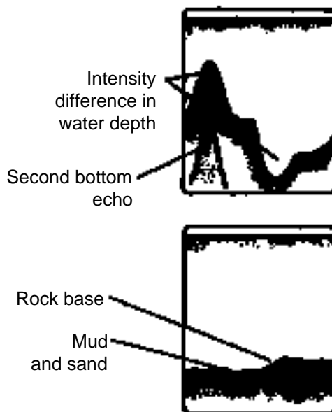
Figure 3-3 Bottom echoes
