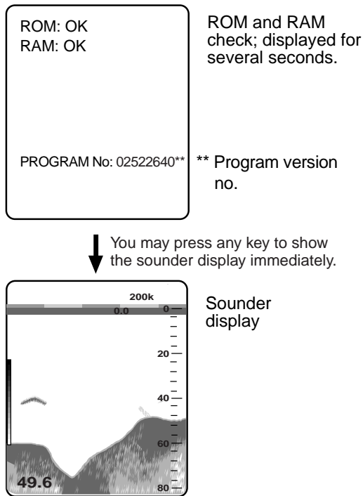
Figure 1-3 Start-up sequence
