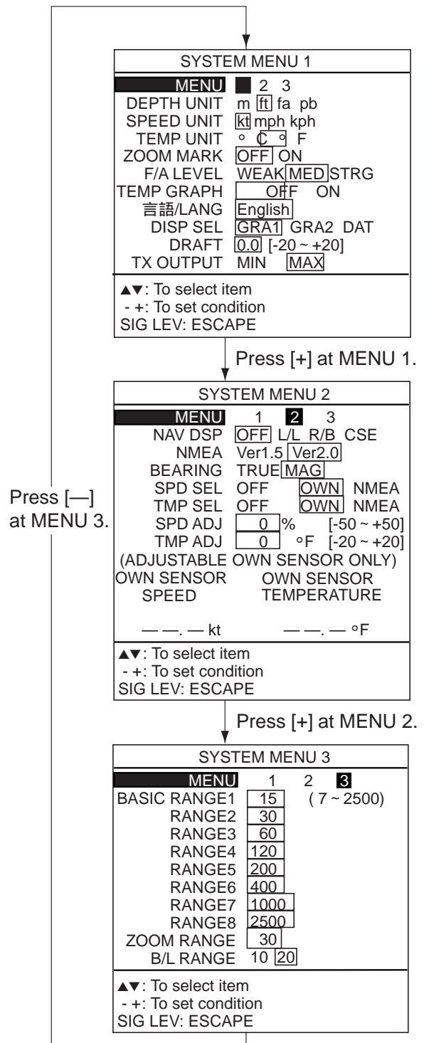
Figure 2-2 System menus
