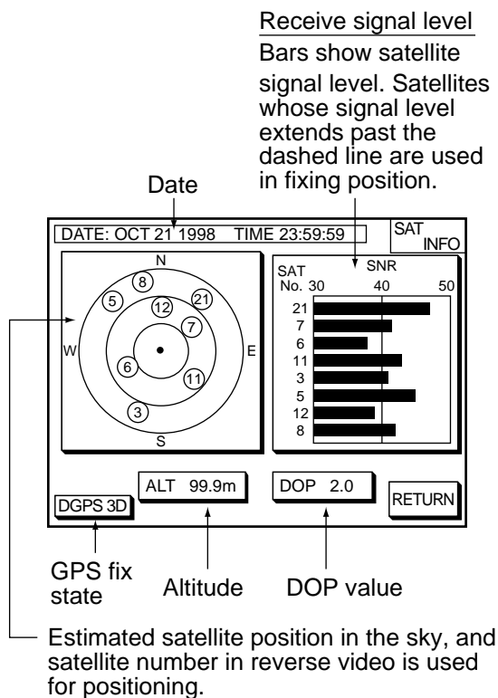
Figure 2-11 GPS satellite monitor display
